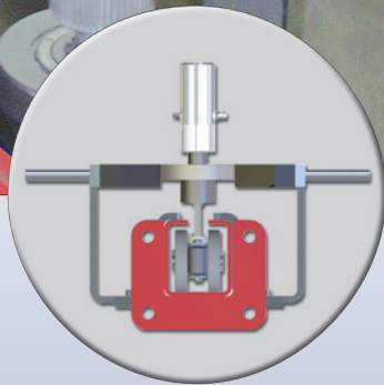
Sectional view -VLD
